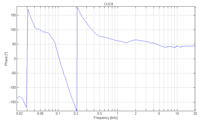
CUC8 PHASE FREQUENCY RESPONSE
