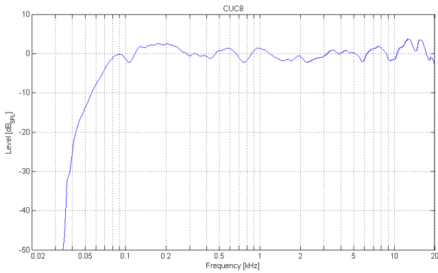
CUC8 UNPROCESSED FREQUENCY RESPONSE
