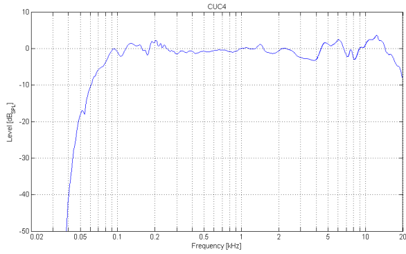
CUC4 UNPROCESSED FREQUENCY RESPONSE
