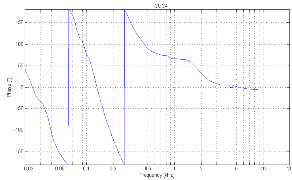
CUC4 PHASE FREQUENCY RESPONSE
